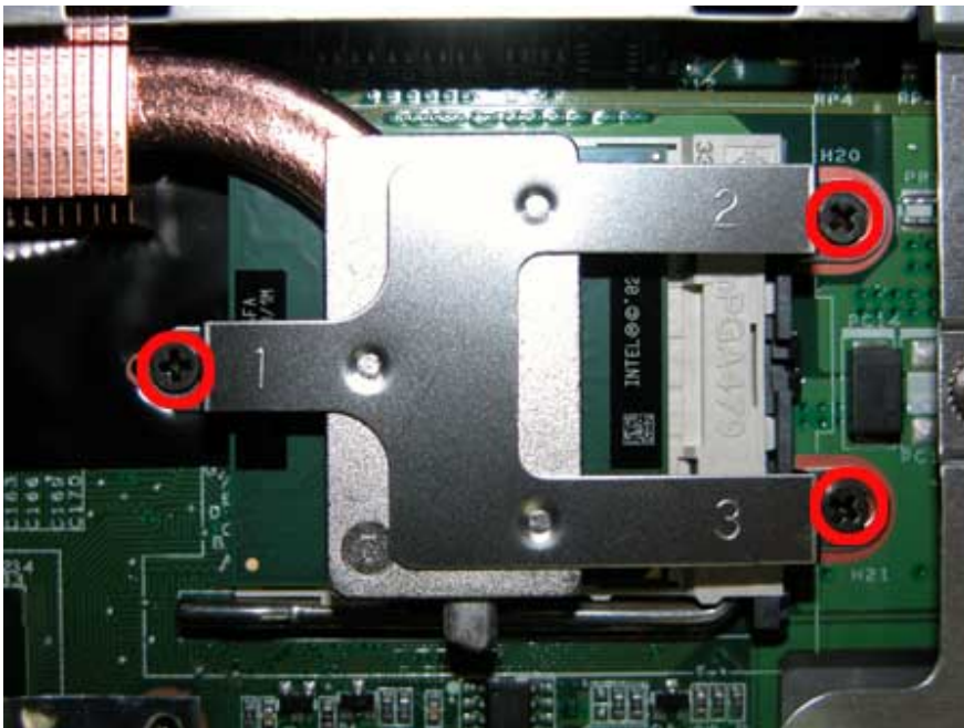
Fig. 22 CPU Heat Sink
